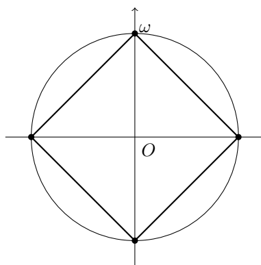
n = 4, \omega = i
