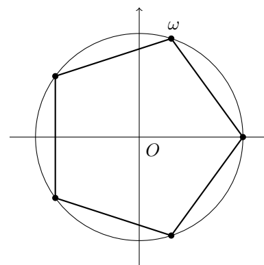
n = 5, \omega = e^{2i\pi/5}
