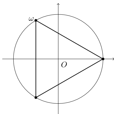
n = 3, \omega = j
